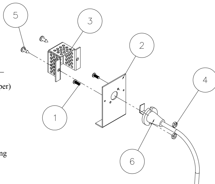
UPPER ASSEMBLY
