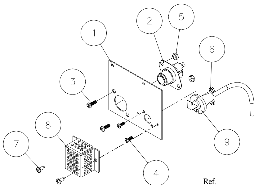
LOWER ASSEMBLY
